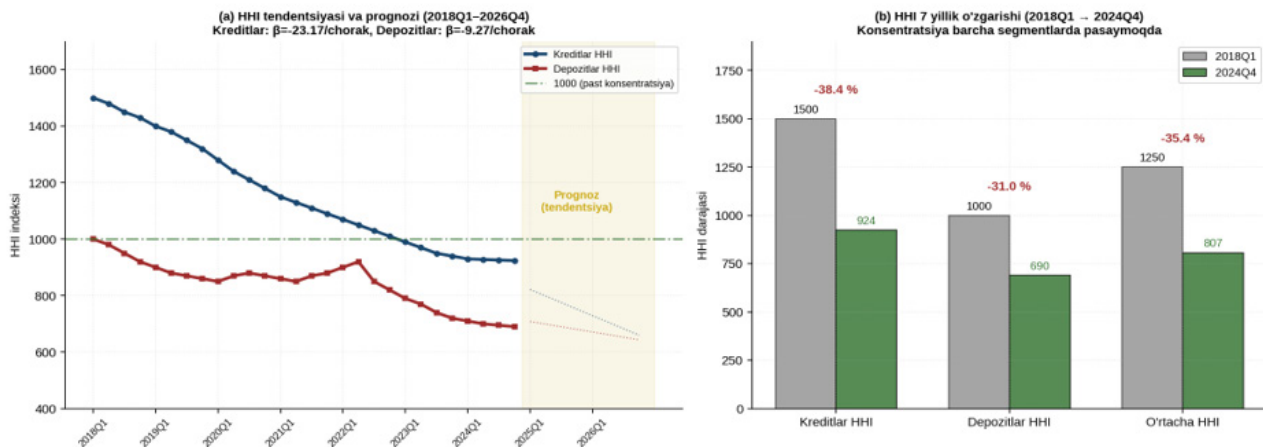
Figure 3. Quarterly evolution of HHI and forecast (2018Q1–2026Q4) 24
